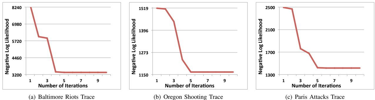
Figure 5. Convergence Analysis of HA-EM
