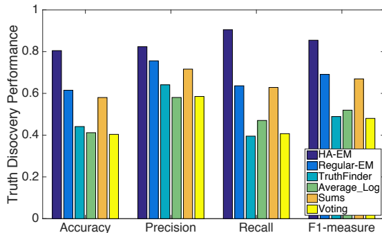
Figure 4. Evaluation on Paris Terrorist Attacks Trace
