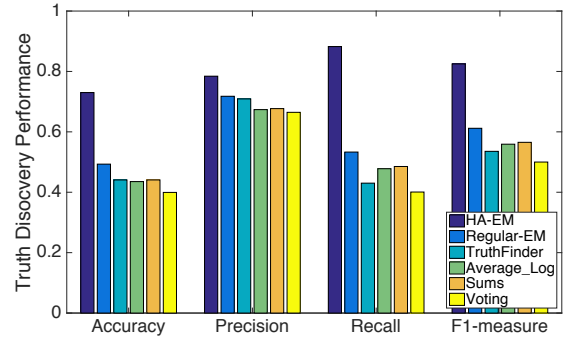
Figure 2. Evaluation on Baltimore Riots Trace
