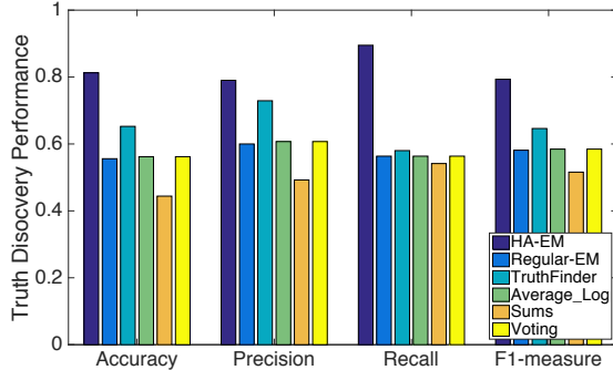
Figure 3. Evaluation on Oregon Shooting Trace
