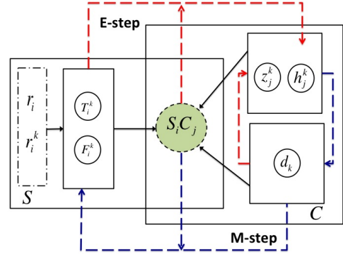
Figure 1. The E and M steps of HA-EM Scheme
